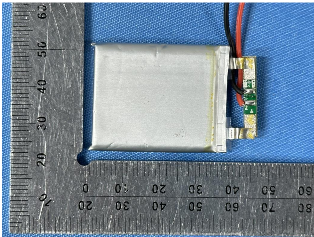
Fig.14 –Battery view
