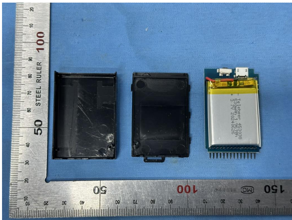
Fig.6– Internal view
