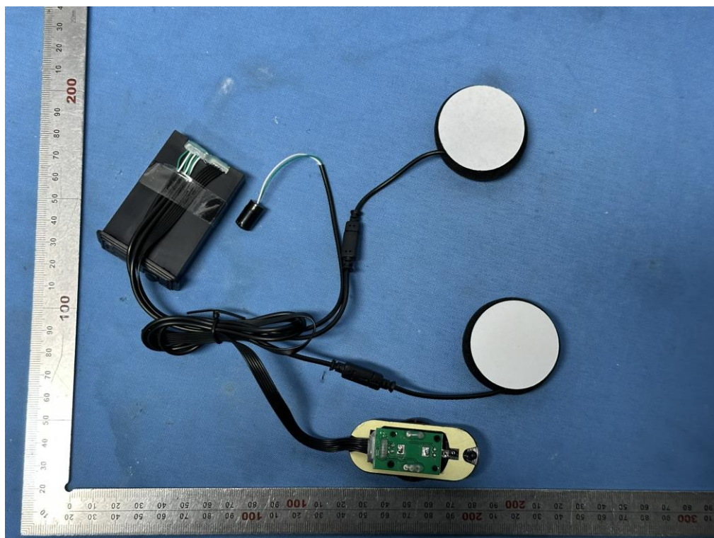
Fig.4 – overall view
