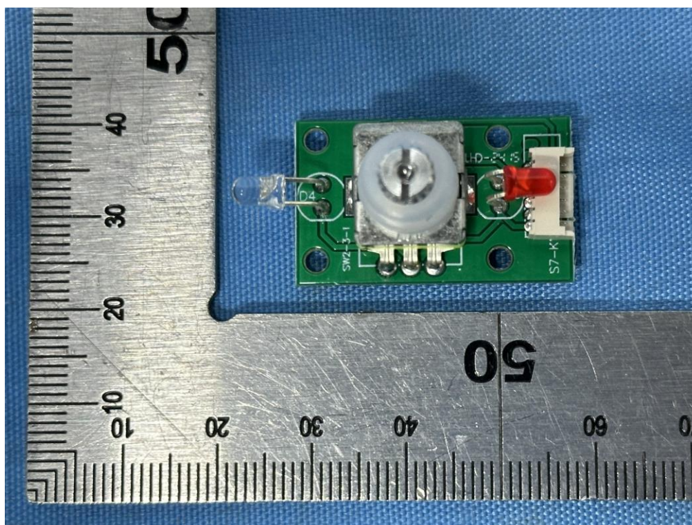
Fig.11- PCB view
