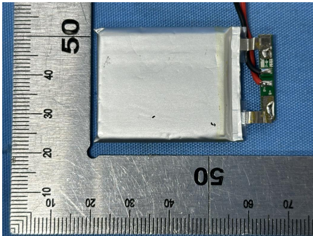
Fig 15 –Battery view
