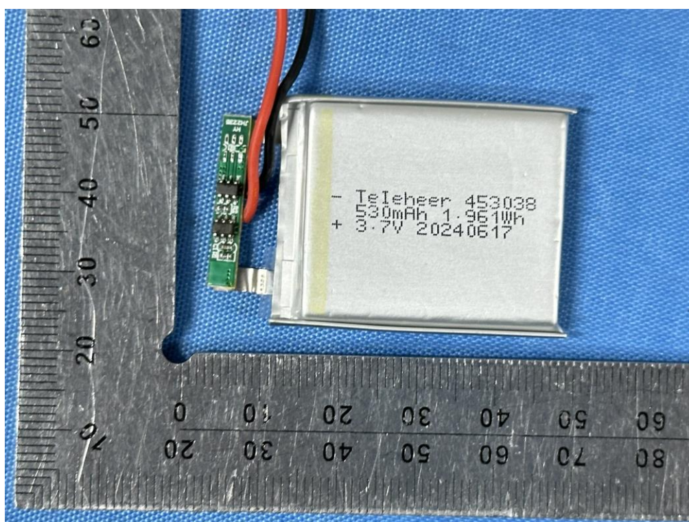
Fig 16 –Battery view
