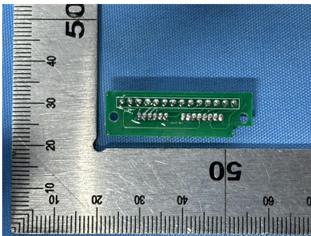
Fig.14 -PCB view
